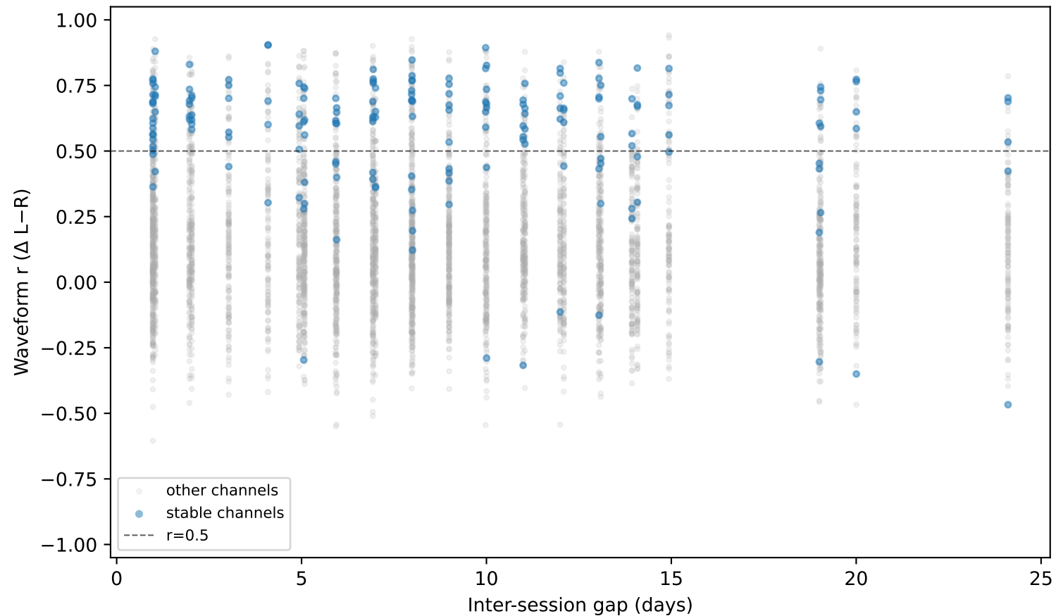
Curius_BgoA | stability across sessions (stable n=6)
