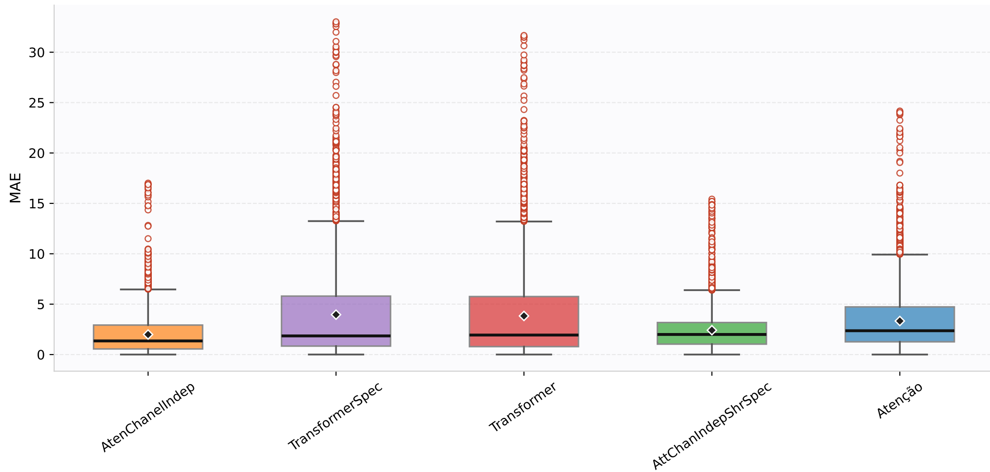
Agregado — MAE — paradigma=first
