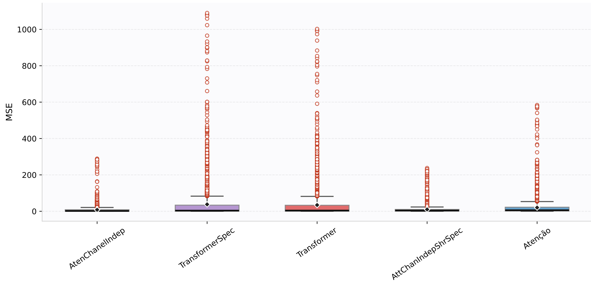
Agregado — MSE — paradigma=first
