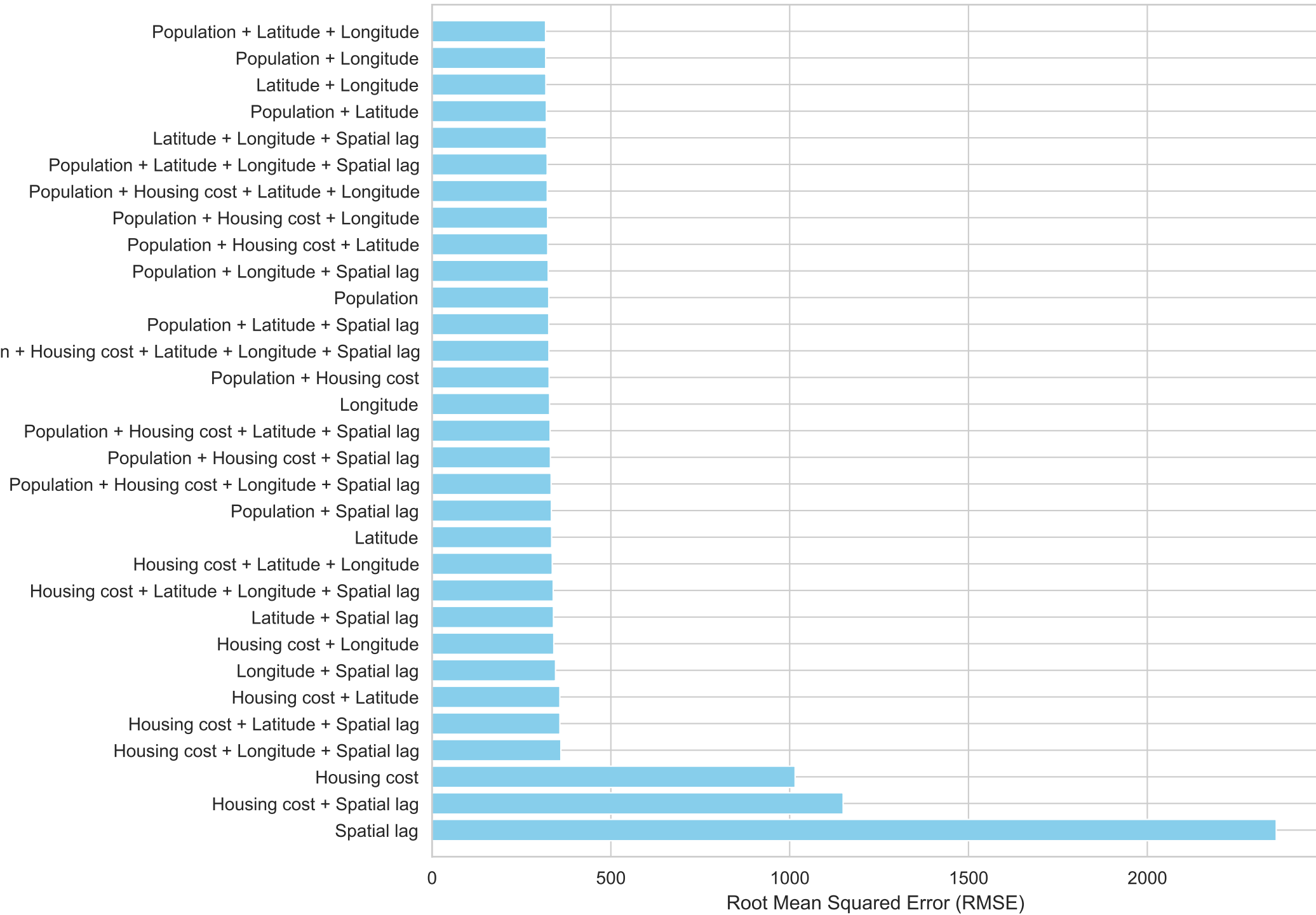
Random Forest performance by feature combination
