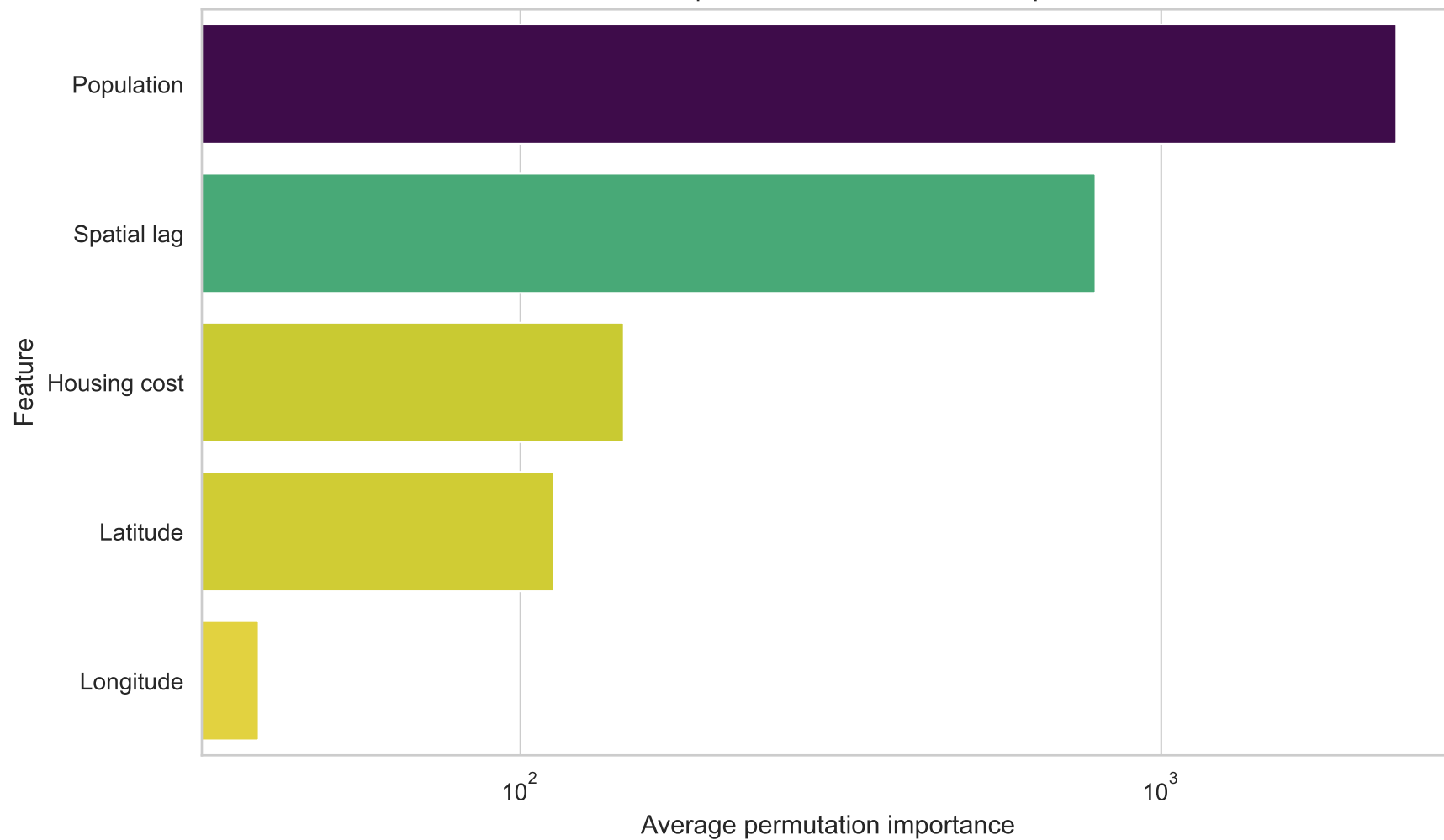
Random Forest permutation-based feature importances
