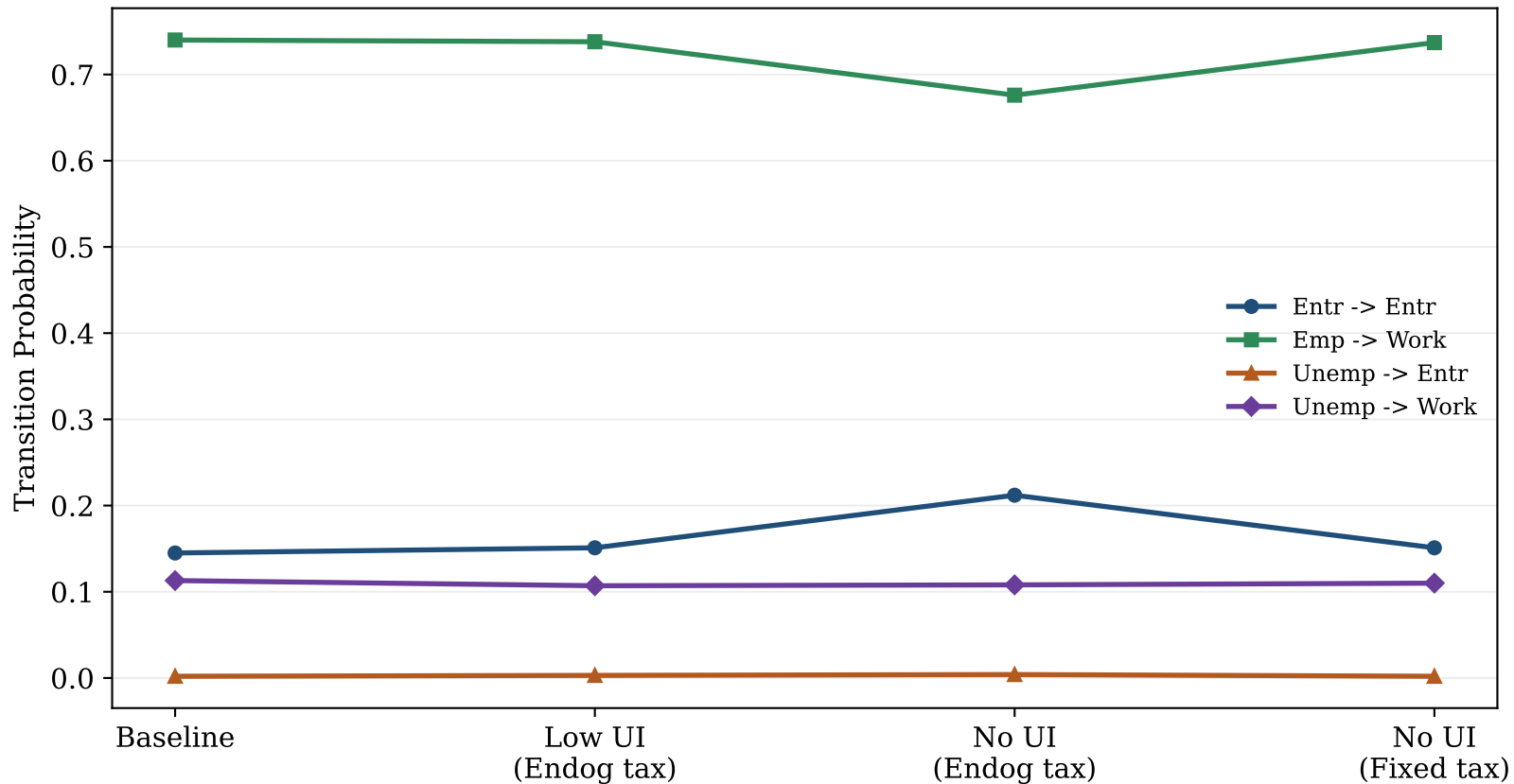
Key Transition Rates Across Current Experiments
