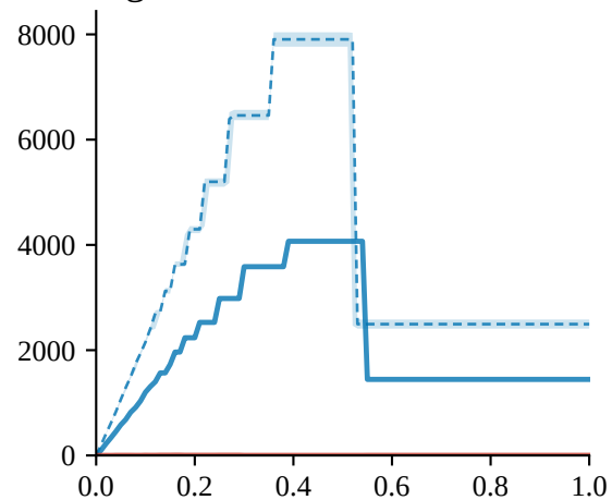
human_long (w=3)
