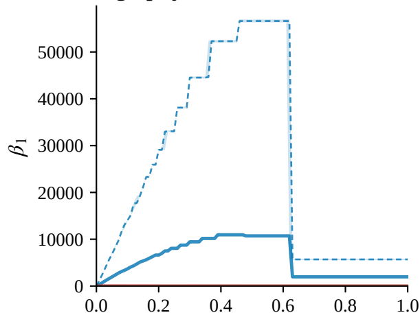
tags-physics
