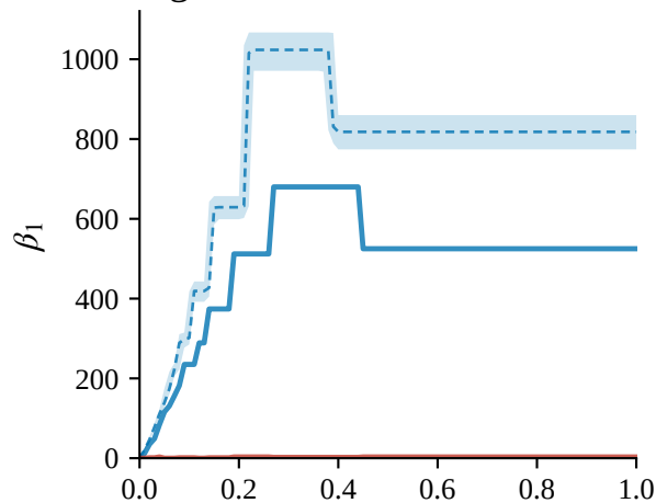
tags-physics
