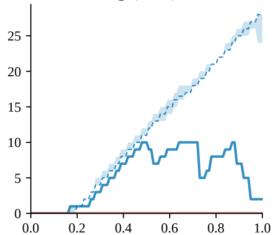
human_long (w=3)
