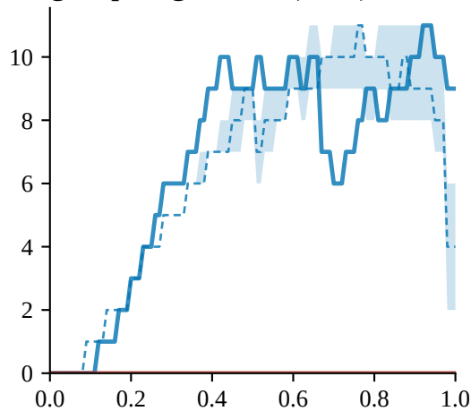
group_regulation (w=3)
