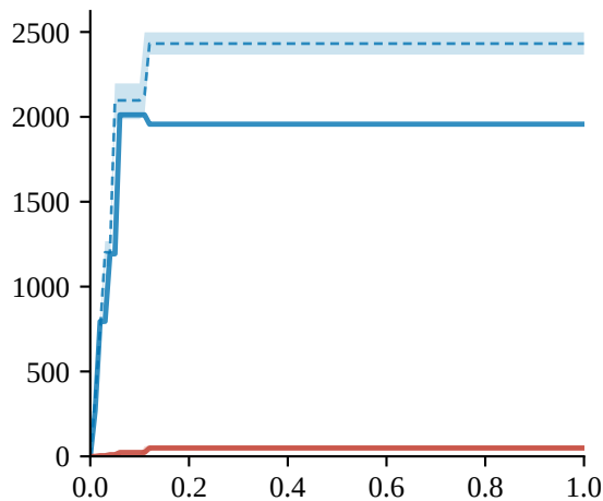
group_regulation (w=3)
