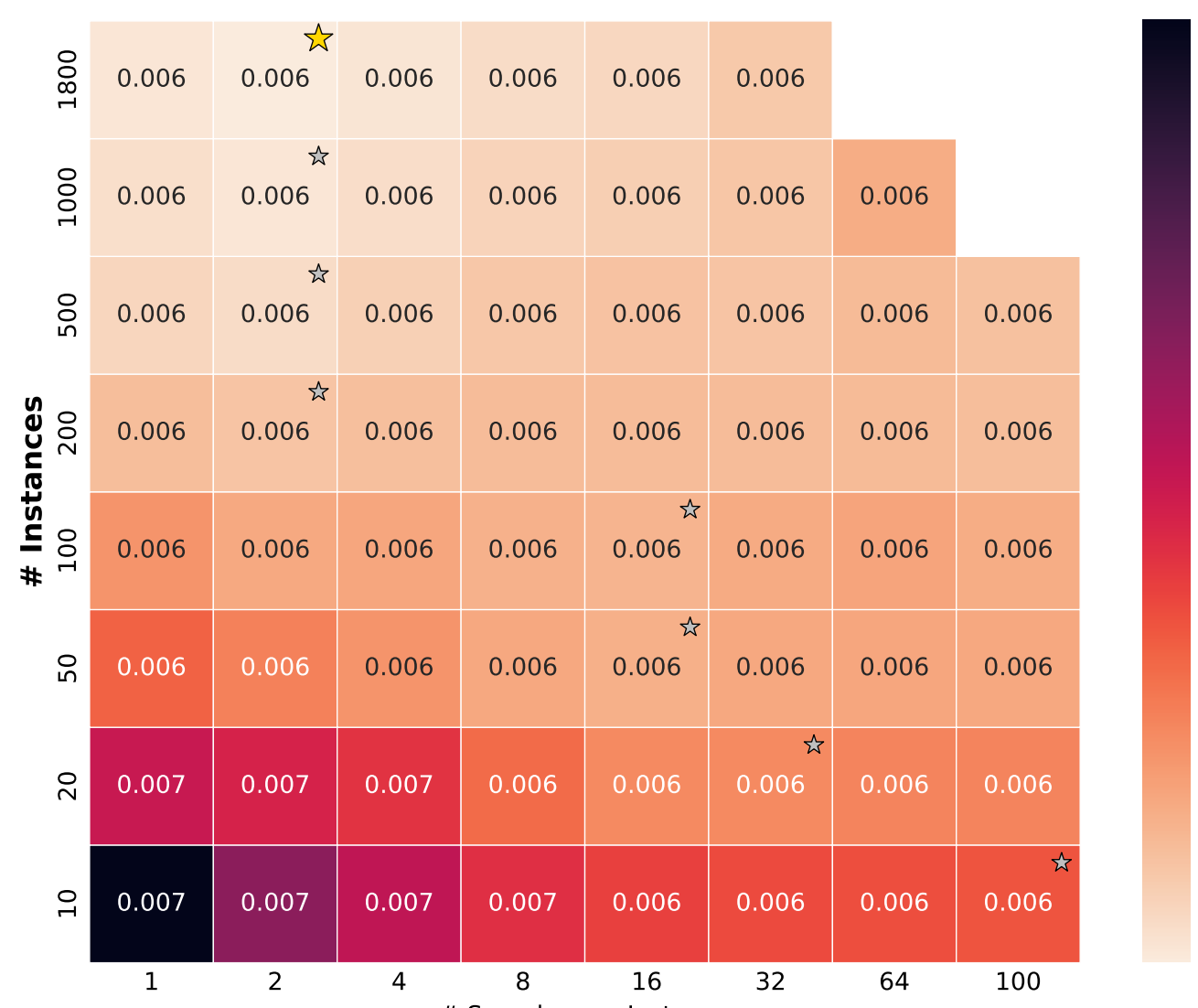
CRPS
