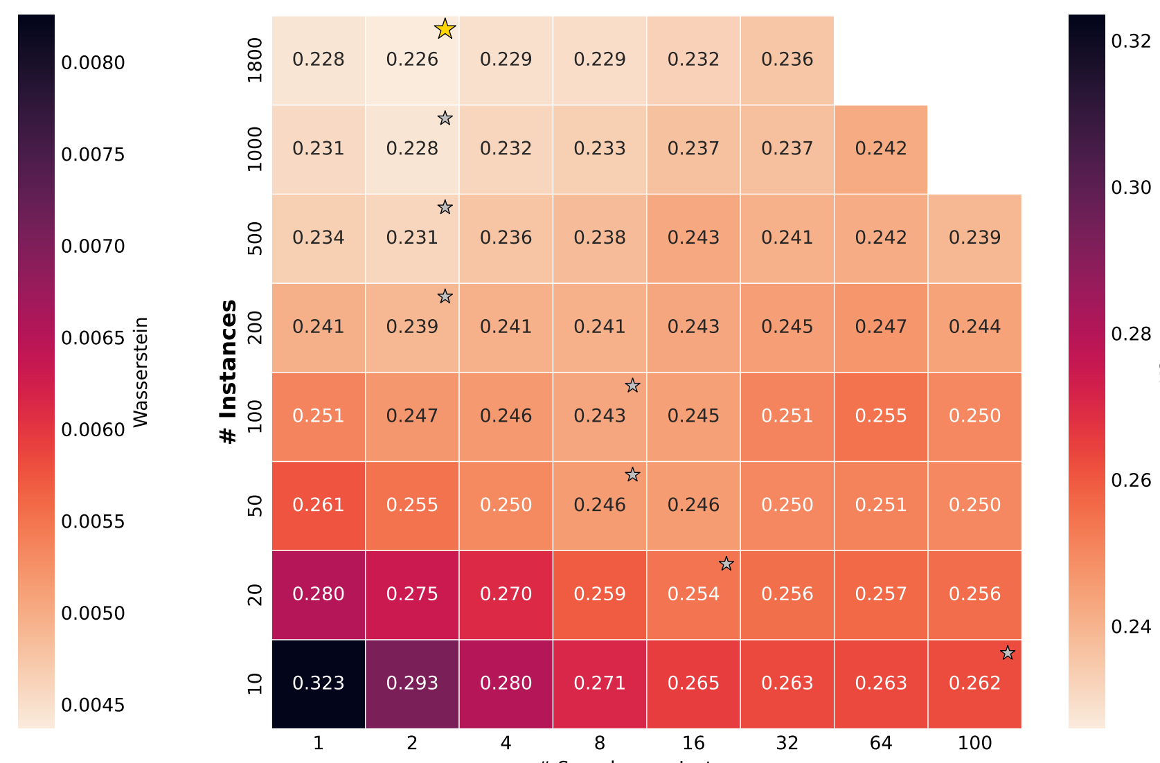
KS
