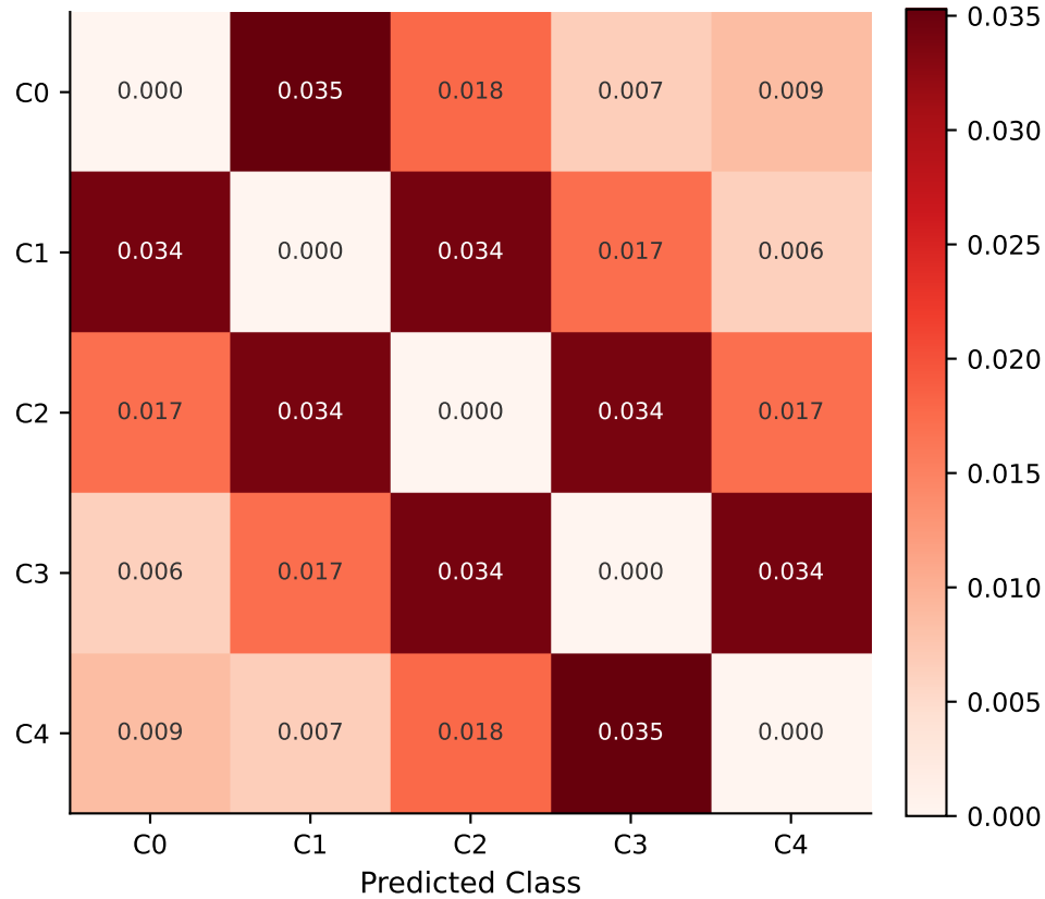
TabPFN Flat
