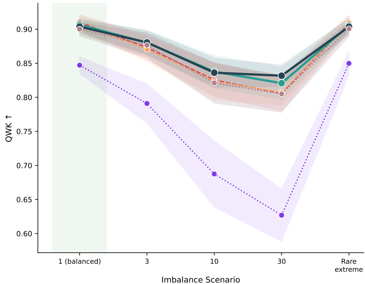
Severe Misranking Rate and QWK under Increasing Class Imbalance
