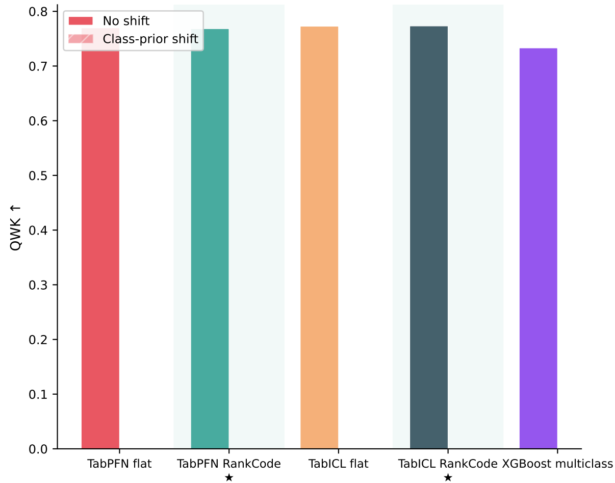
Distribution Shift Robustness (class-prior shift, 46 datasets, 5 splits)
