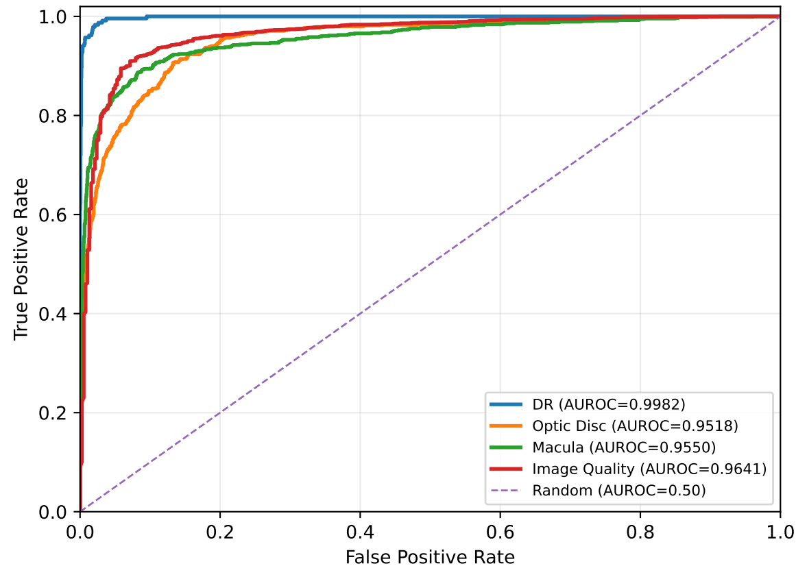
ROC curves for the four primary labels (Protocol 1, T=20, seed 42, n=3,266)
