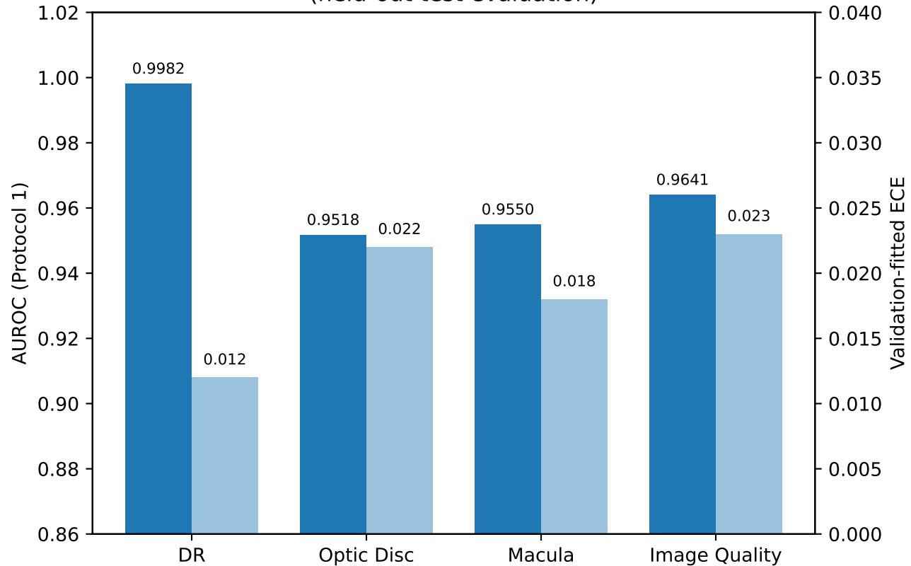
AUROC and validation-fitted ECE (held-out test evaluation)
