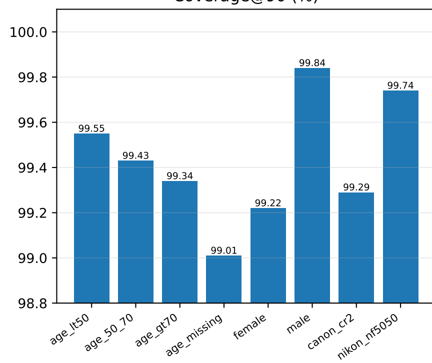
Coverage@90 (%)
