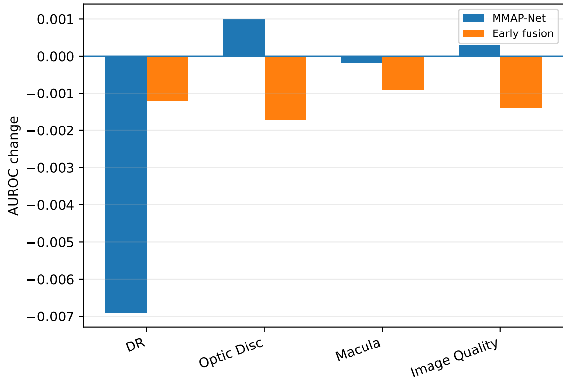
Signed AUROC change
