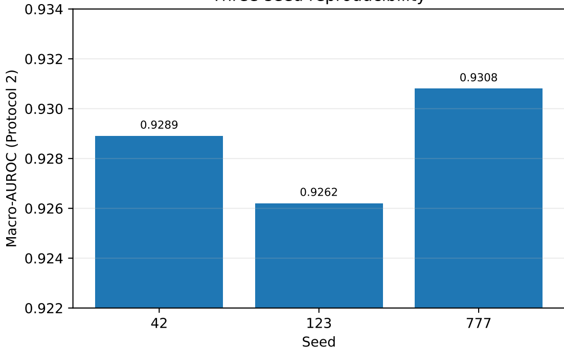
Three-seed reproducibility
