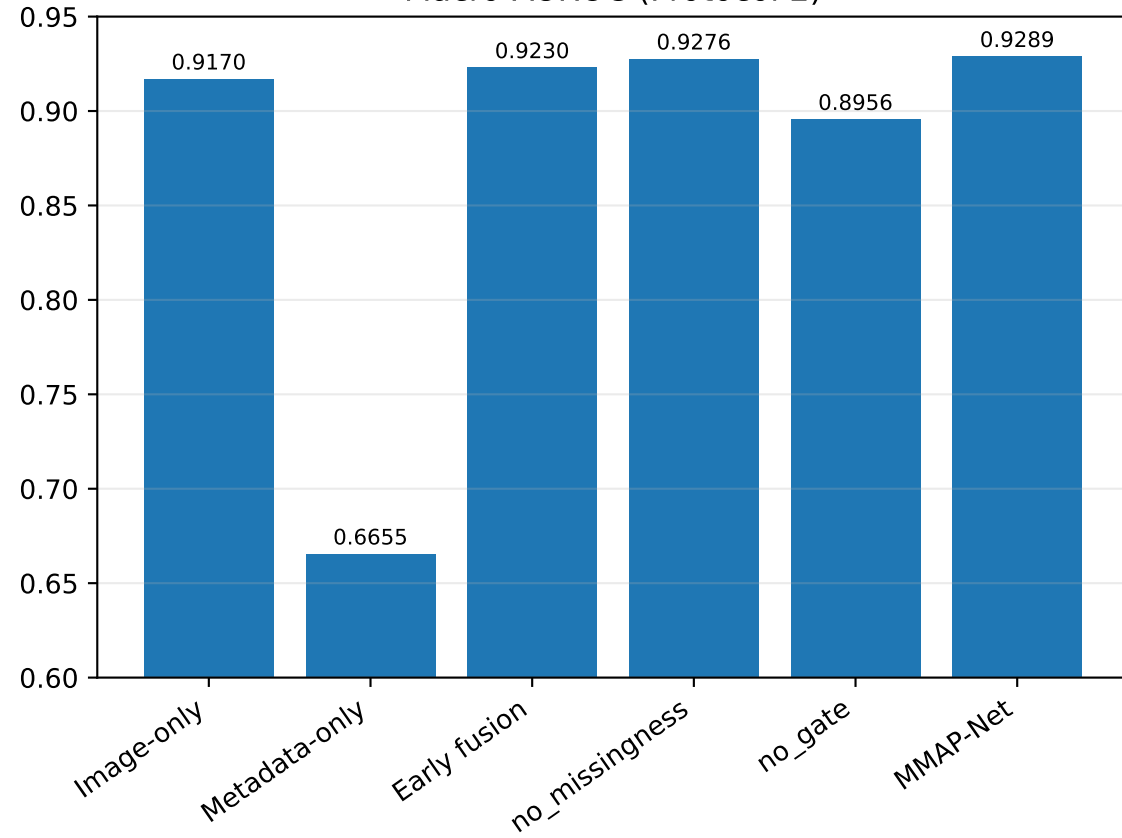
Macro-AUROC (Protocol 2)
