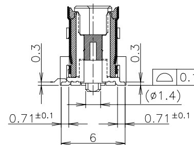
SECT. Z-Z (SIGNAL POSITION)
