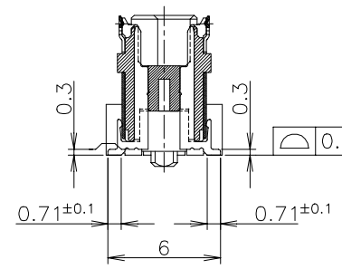
SECT. Y-Y (GROUND POSITION)
