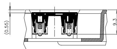
SECT. D-D (SCALE 2:1) ROTATED 90° CW
