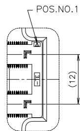
DETAIL F (SCALE 2:1)
