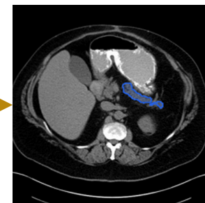
Segmentation output
