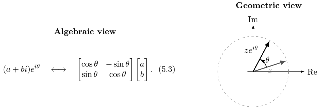
Figure 2: Multiplication by e^{i\theta} rotates a complex coefficient while preserving its magnitude. Fourier time evolution uses exactly this operation to advance phase.
