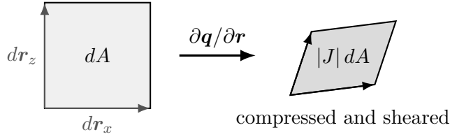
Figure 3: Locally, the Jacobian maps the parameter-space basis vectors and scales their enclosed area by |J| . Compression corresponds to 0 < J < 1 .
