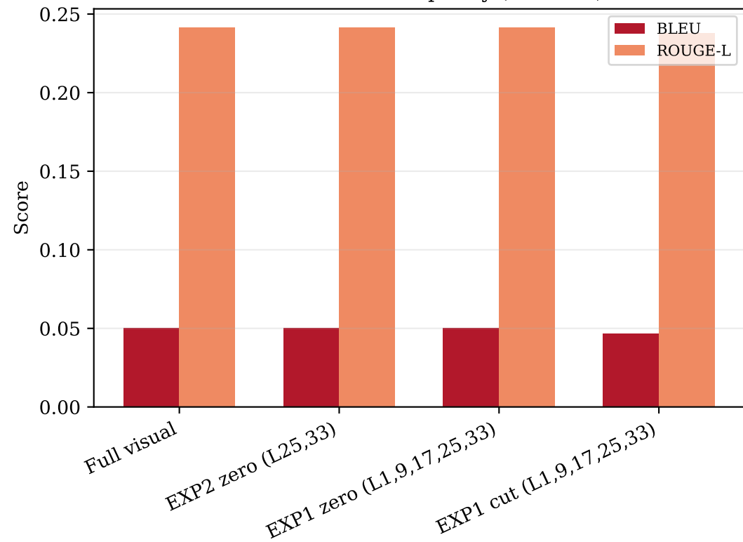
VDC50 — DFlash quality (llava68k)
