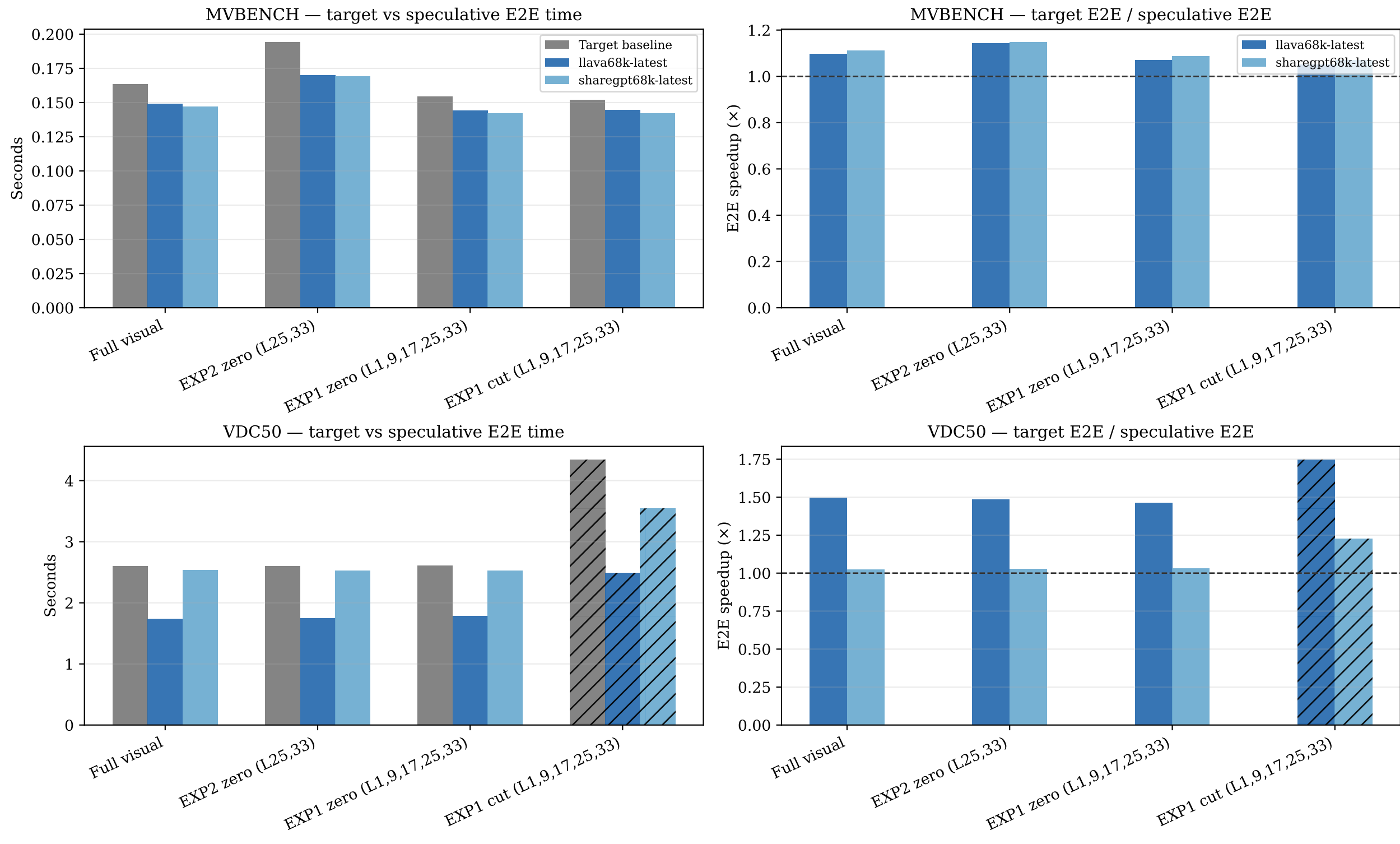
Figure 5. Speculative inference time and end-to-end speedup (hatched VDC bars = cross-GPU exploratory comparison)
