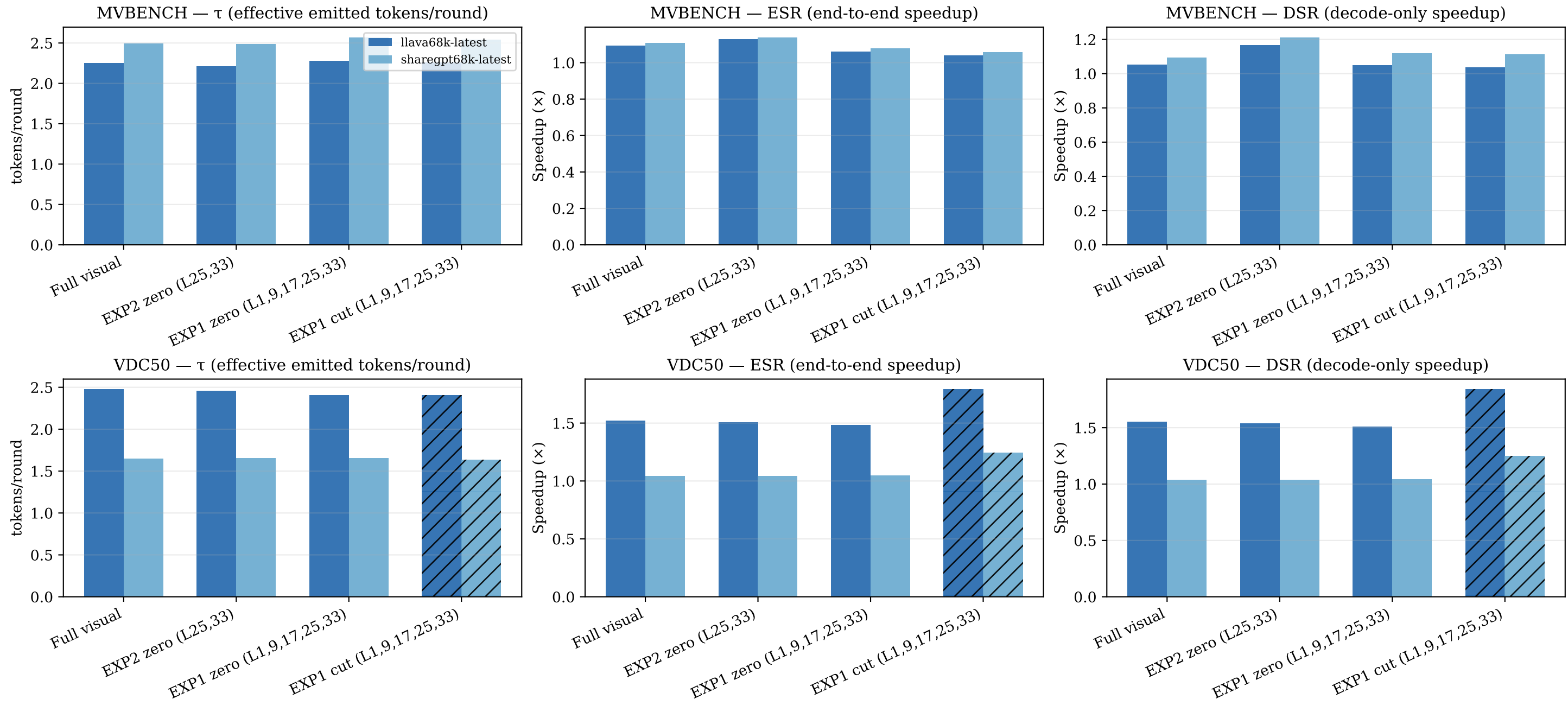
Figure 6. Speculative acceptance and speedup statistics (hatched VDC bars = cross-GPU exploratory comparison)
