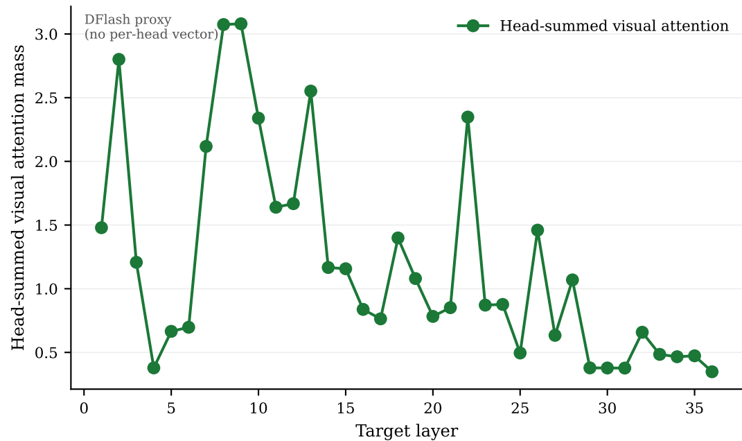
(b) Layer-wise visual attention
