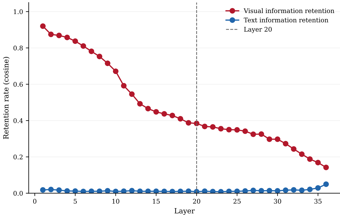
Figure 6. Layer-wise information retention (DFlash proxy)
