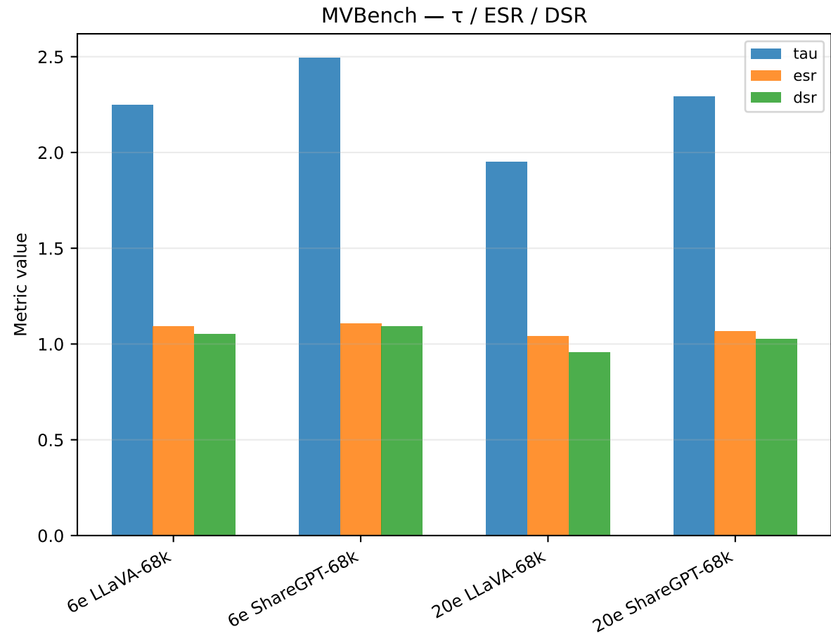
Figure 3. MVBench speculative performance (same GPU)
