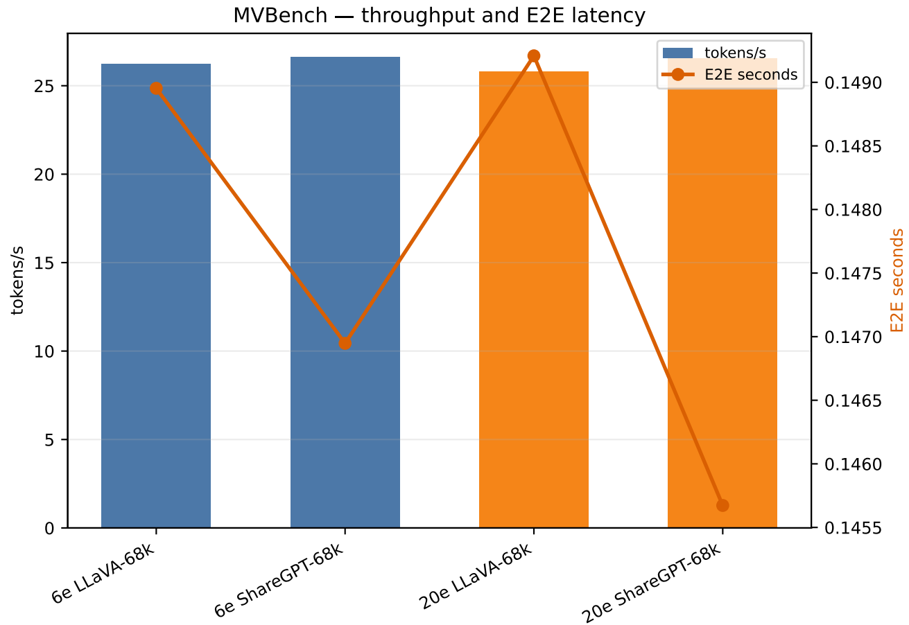
Figure 3. MVBench speculative performance (same GPU)
