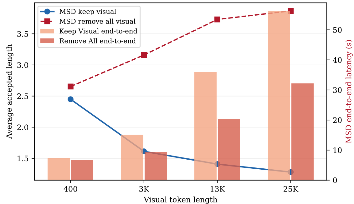
(a) MSD visual-length sweep (VDC-50 local)
