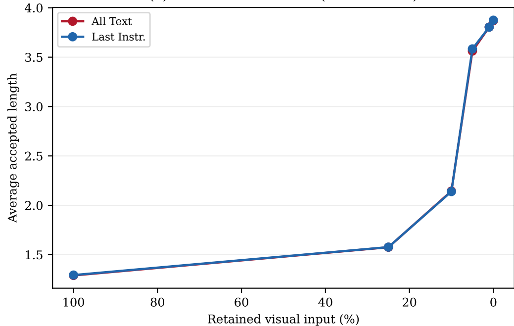
(b) Draft visual retention (VDC-50 local)
