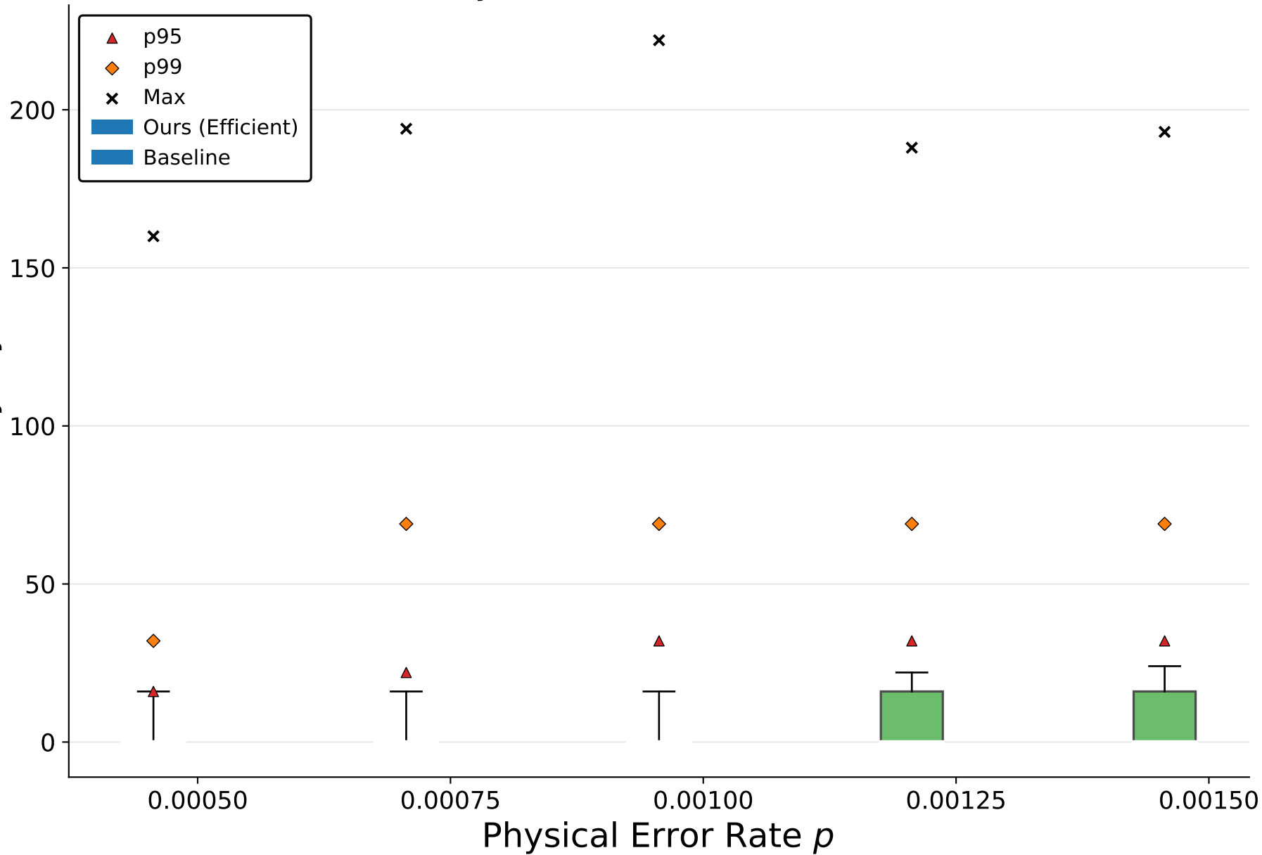
Latency Distribution Box Plot (L=3)
