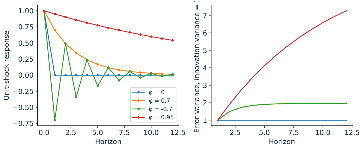
Figure 1: A unit shock can alternate while error variance remains positive. These curves are analytic, with innovation variance one.
