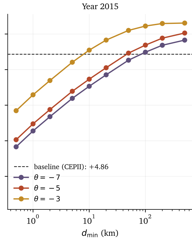
Gravity-regression home-bias coefficient \hat{\gamma} across regularization grain and structural \theta (BACI-CEPII panel, \log X_{ij} = \alpha + \beta \log d_{ij} + \gamma \mathbf{1}\{i = j\} + \eta_i + \mu_j )
