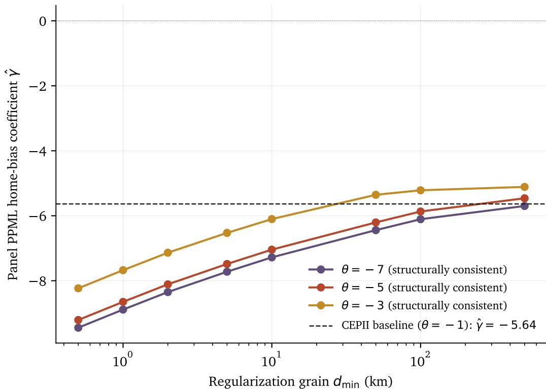
Pooled panel PPML home-bias coefficient \hat{\gamma} vs d_{\min} , structurally consistent \theta , 2010-2015-2020 stacked
