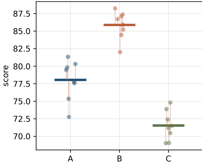
Within-group variation (observations vs.\ group mean)
