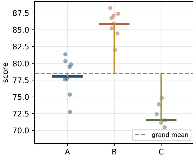
Between-group variation (group means vs.\ grand mean)
