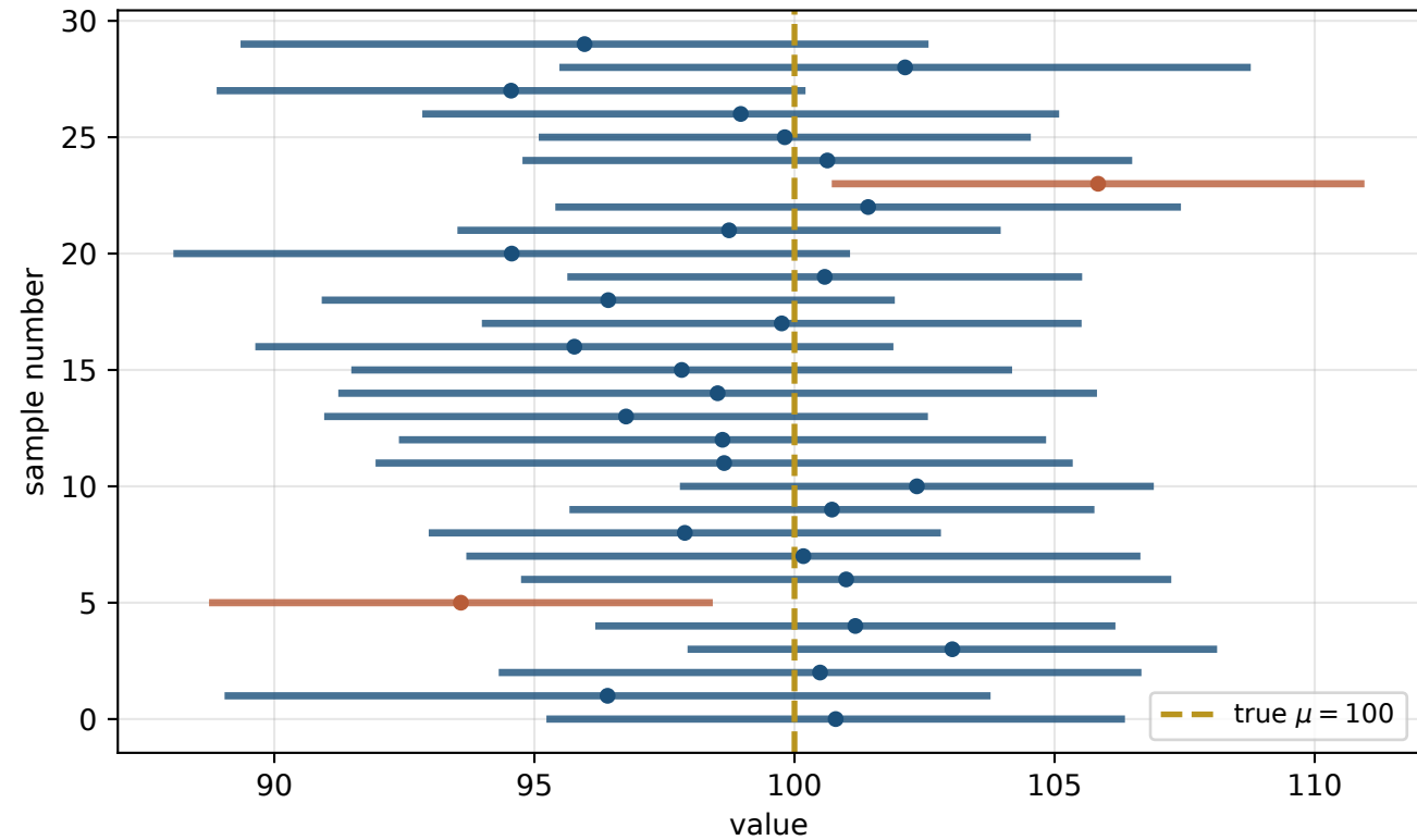
30 samples, 30 confidence intervals: 28 contain \mu
