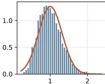
\bar{X} for n = 10
