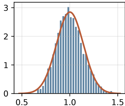
\bar{X} for n = 50
