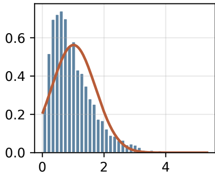
\bar{X} for n = 2
