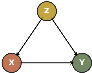
Confounder Z (condition on Z)
