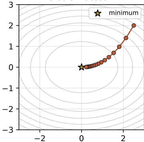
Gradient descent
