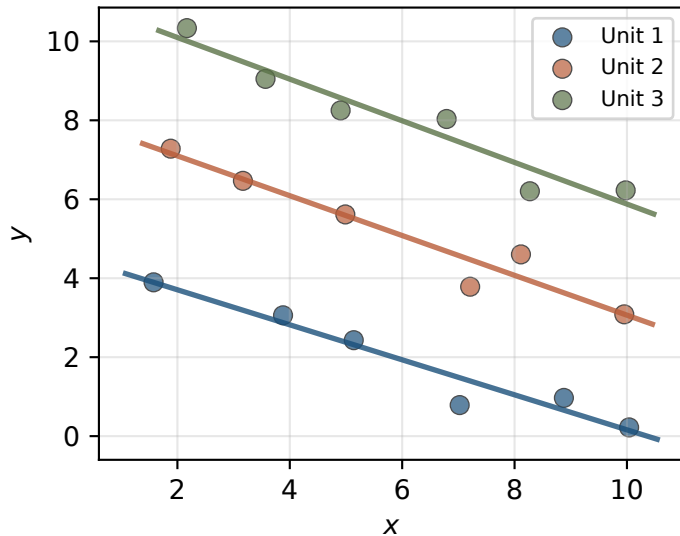
FE: within-unit slope \approx -0.5
