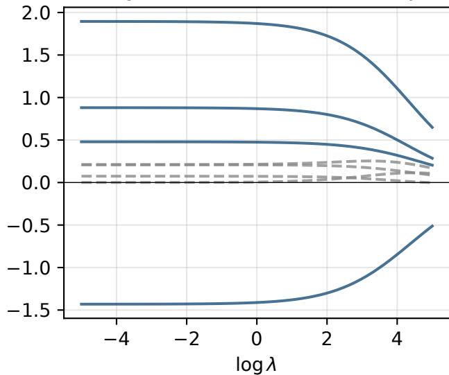
Ridge: coefficients shrink smoothly
