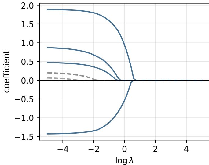
Lasso: coefficients hit zero
