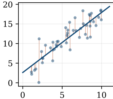
SS_{\text{res}} : residual
