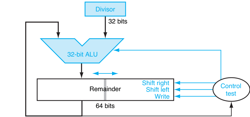
FIGURE 3.12 An improved version of the division hardware. The Divisor register, ALU, and Quotient register are all 32 bits wide, with only the Remainder register left at 64 bits. Compared to Figure 3.9, the ALU and Divisor registers are halved and the remainder is shifted left. This version also combines the Quotient register with the right half of the Remainder register. (As in Figure 3.6, the Remainder register should really be 65 bits to make sure the carry out of the adder is not lost.)
