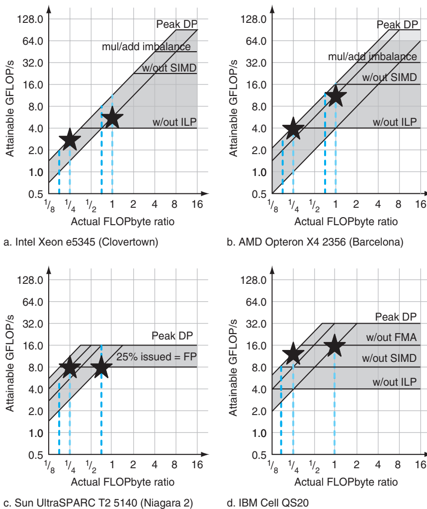
FIGURE 7.19 Roofline model for multicore multiprocessors in Figure 7.15. The ceilings are the same as in Figure 7.13. Starting from the upper left hand corner, the computers are: (a) Intel Xeon e5345 (Clovertown), (b) AMD Opteron X4 2356 (Barcelona), (c) Sun UltraSPARC T2 5140 (Niagara 2), and (d) IBM Cell QS20. Note the ridge points for the four microprocessors intersect the X-axis at the arithmetic intensities of 6, 4, 1/3 , and 3/4 , respectively. The dashed vertical lines are for the two kernels of this section and the stars mark the performance achieved for these kernels after all the optimizations. SpMV is the pair of dashed vertical lines on the left. It has two lines because its arithmetic intensity improved from 0.166 to 0.255 based on register blocking optimizations. LBHMD is the dashed vertical lines on the right. It has a pair of lines in (a) and (b) because a cache optimization skips filling the cache block on a miss when the processor would write new data into the entire block. That optimization increases the arithmetic intensity from 0.70 to 1.07. It's a single line in (c) at 0.70 because UltraSPARC T2 does not offer the cache optimization. It is a single line at 1.07 in (d) because Cell has local store loaded by DMA, so the program doesn't fetch unnecessary data as do caches.
