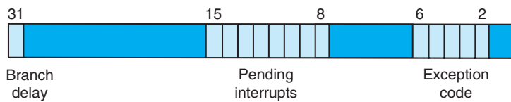
FIGURE B.7.2 The Cause register.
