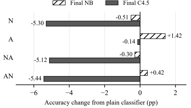
Fig. 1. Protocol B mean accuracy change from the corresponding plain classifier, with equal dataset weight. N is filtering, A is attribute weighting, and NA/AN are the combined orders. Negative values mean lower accuracy. These are descriptive differences, not significance tests.
