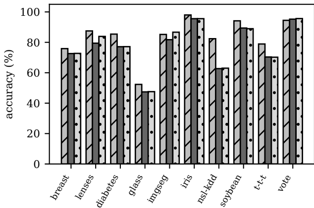
Algorithm 2 (hybrid NB)
