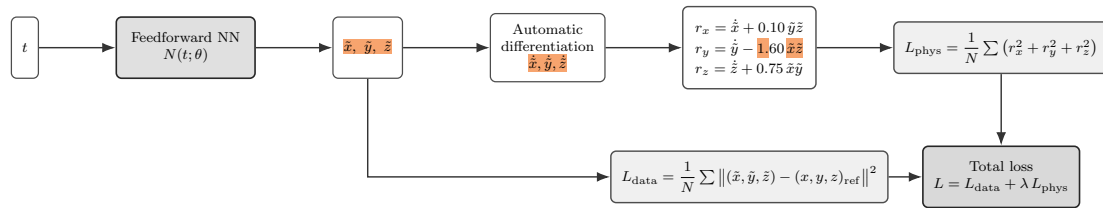
Figure 2.2: Architecture of a Physics-Informed Neural Network incorporating physical loss [2].
