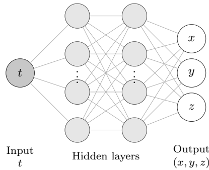
Figure 2.1: Feedforward ANN used in this study. A single scalar input, time t , is propagated through a stack of hidden layers to predict the Lorenz-1960 state (x(t), y(t), z(t)) . The number of hidden layers, the neurons per layer, and the activation function are the axes compared in this work [1].
