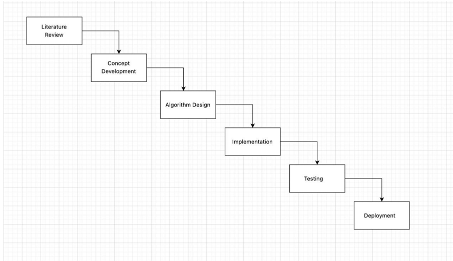
Figure 1.1: Methodology Diagram
