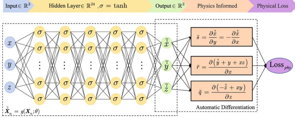
Figure 2.2: Architecture of a Physics-Informed Neural Network incorporating physical loss [2].
