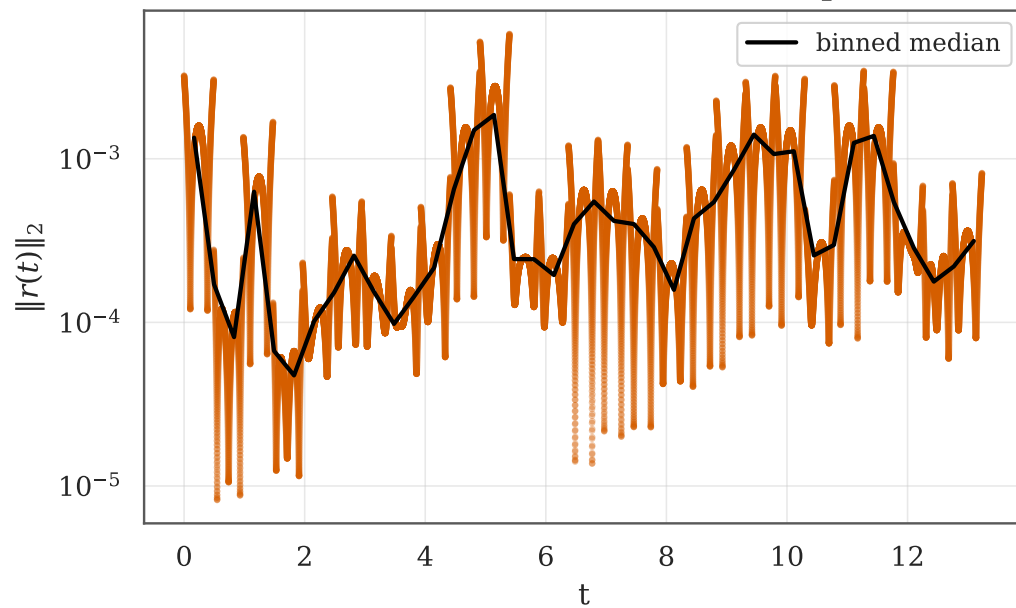
(d) Trained residual at collocation points
