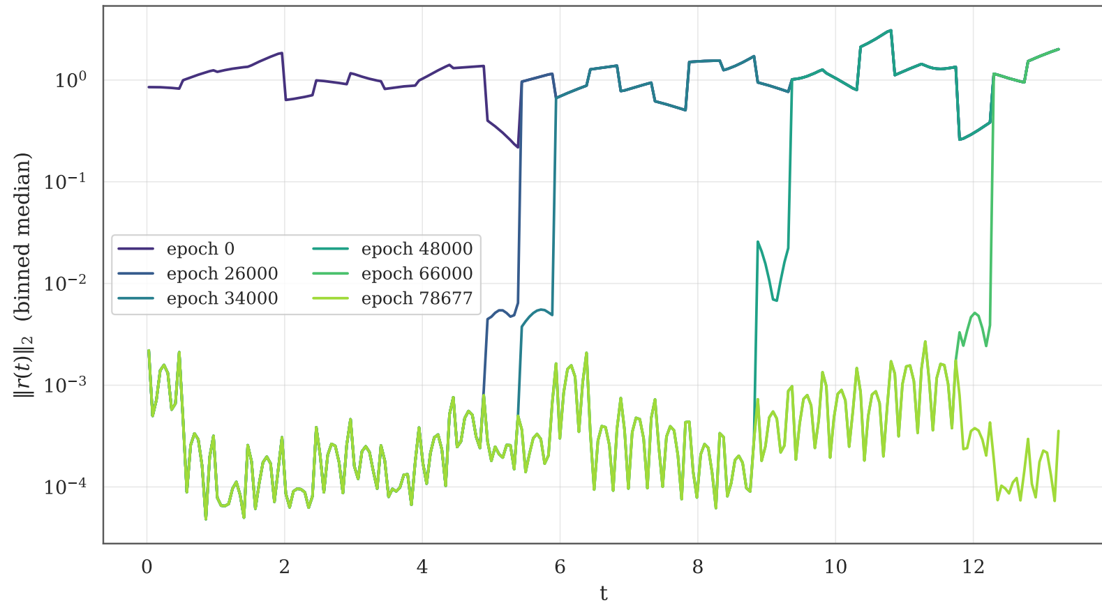
Residual profile by epoch — 4x60 tanh, hard IC, 39793 uniform points, 27 windows, causal
