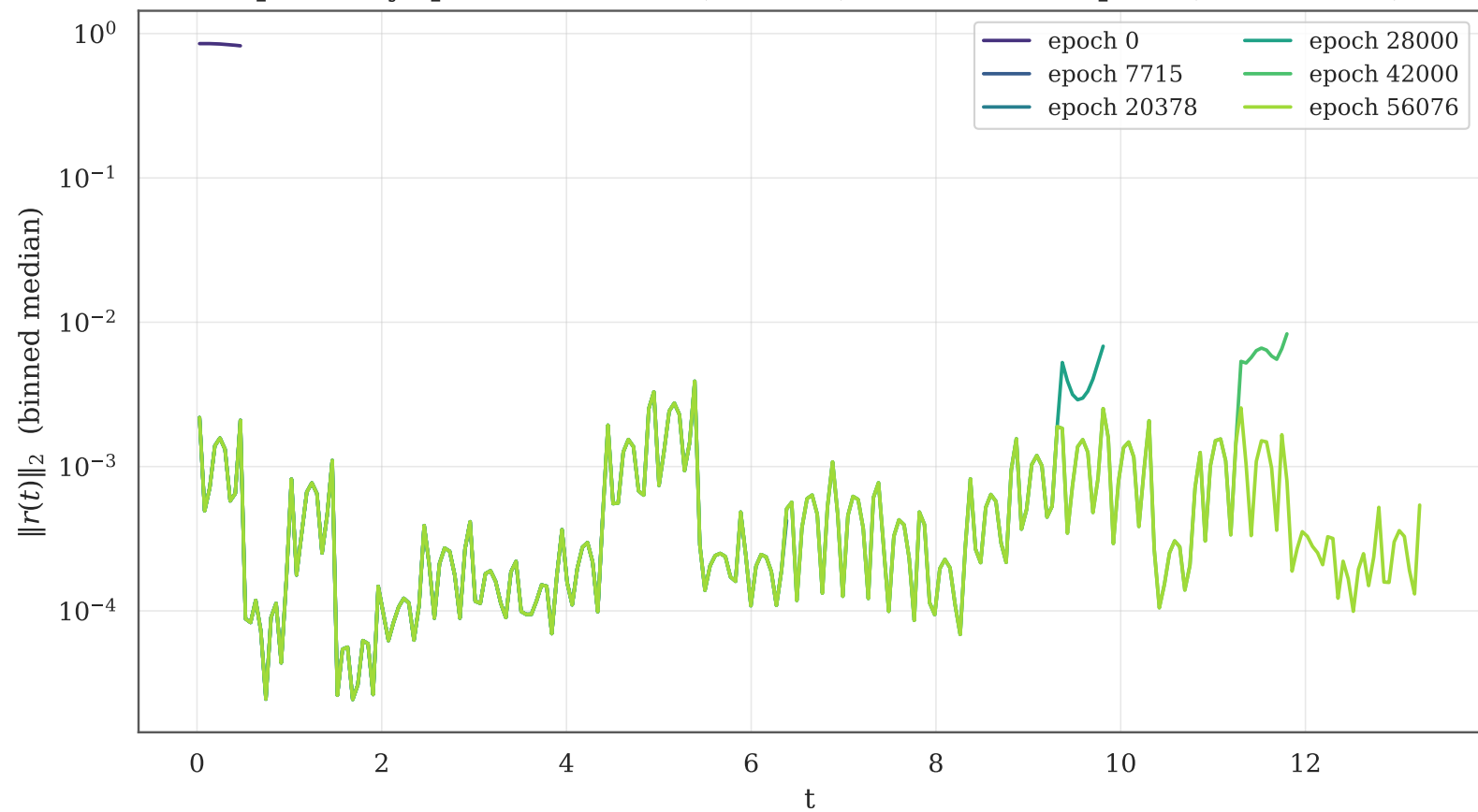
Residual profile by epoch — 4x60 tanh, hard IC, 40474 uniform points, 27 windows, causal
