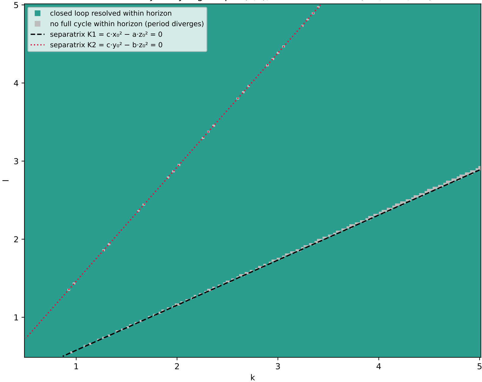
Lorenz-1960 trajectory regime per (k, l), same initial state (0.5, 0.75, 1.0)
