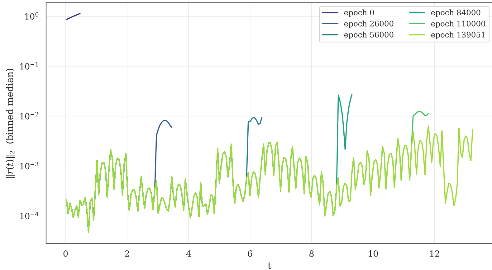
Residual profile by epoch — 4x60 tanh, hard IC, 41446 uniform points, 27 windows, causal
