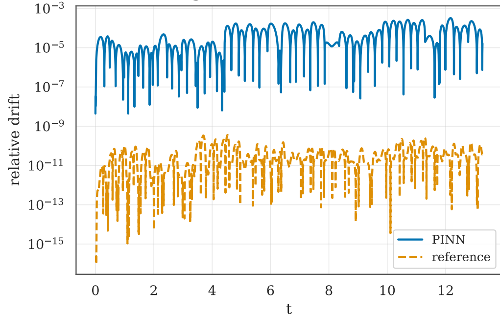
I_2 weights (-0.424, +0.363, +0.830)
