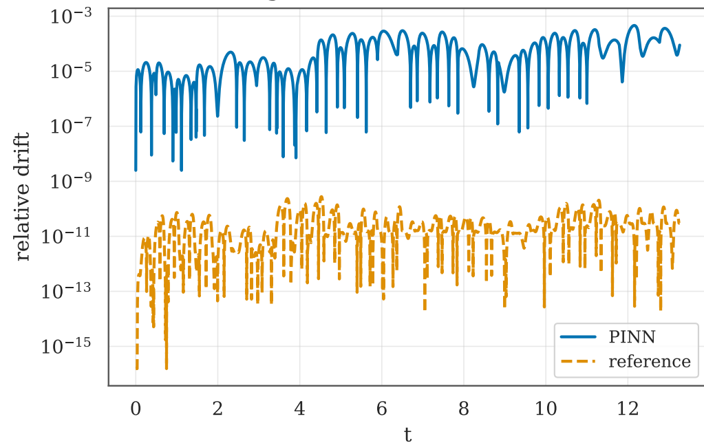
I_1 weights (+0.904, +0.226, +0.363)
